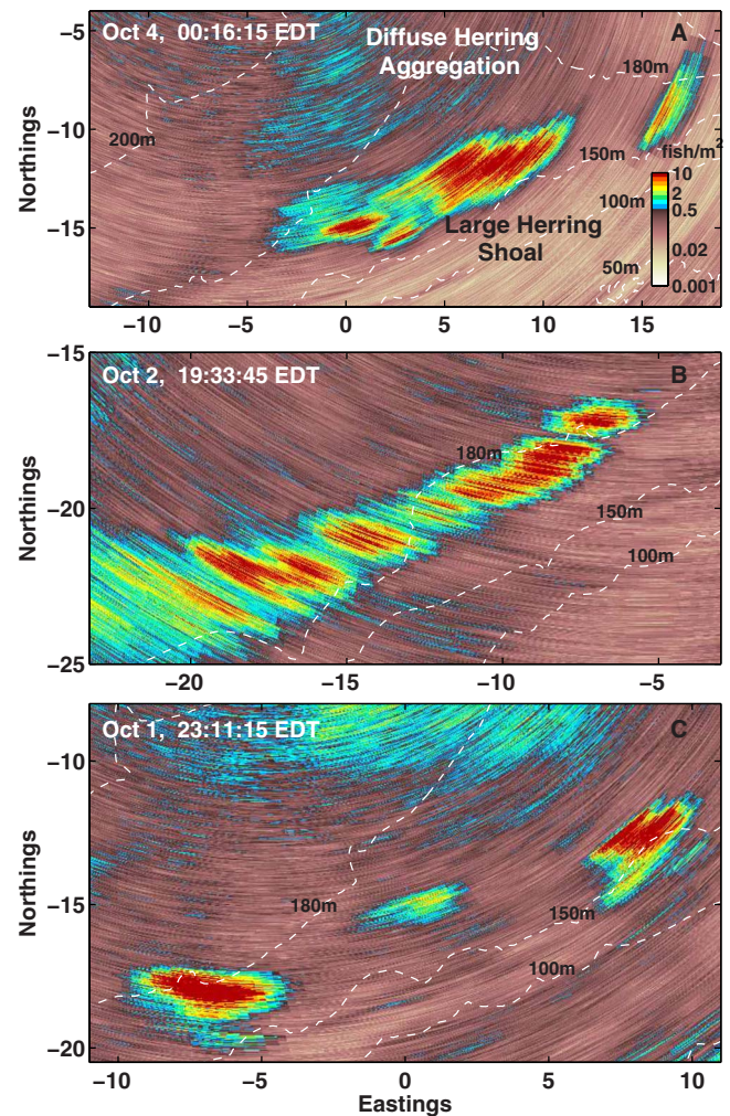
FIG. 2. (Color online) [(A)–(C)] OAWRS images of areal fish density zoomed-in around massive herring shoals, with densities exceeding 10 fish m -2 in population centers. Measured during evening to midnight hours of October 4, 2, and 1, respectively. (A) The total population of herring in the large dense shoal is roughly 170 \times 10^6 , and that in the diffuse cloud outside the large shoal is roughly 70 \times 10^6 . Imaged shoal populations of herring are approximately 86 \times 10^6 and 70 \times 10^6 respectively for (B) and (C). Uncertainty in the abundance estimate is 17–20%. Note that the figures are plotted on different scales, and the coordinate origin is the source location shown in Fig. 1.
